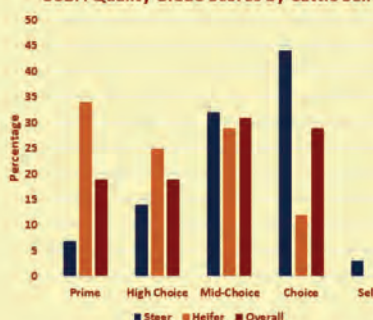
USDA Quality Grade Scores by Cattle Sex
