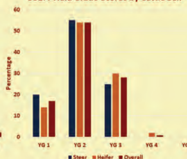
USDA Yield Grade Scores by Cattle Sex
